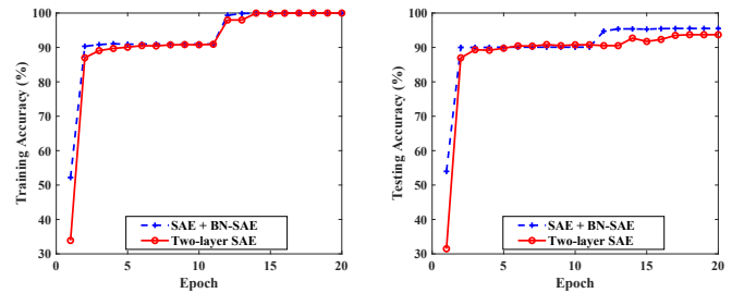
Fig. 8: Training accuracy and testing accuracy. The left figure shows the training accuracy and the right one demonstrates the testing accuracy.
