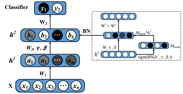
Fig. 4: Structure of the evaluation model.
