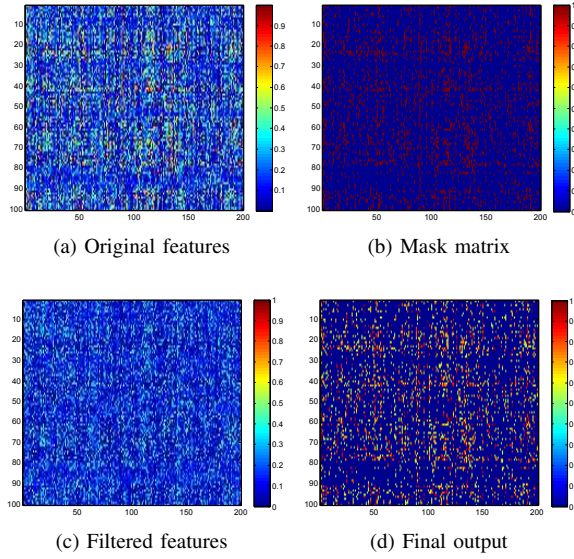
Fig. 3: Filtered features by the BN-based mask matrix.
